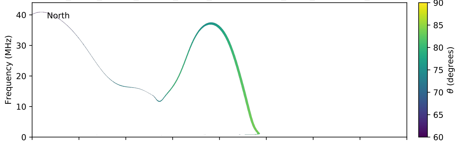
expres_earth_jupiter_europa_jrm09_lossc-wid1deg_3kev_20040213_v11.cdf
