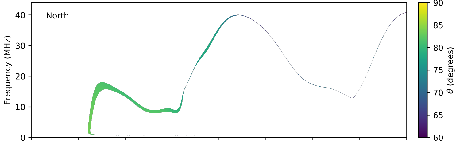
expres_earth_jupiter_europa_jrm09_lossc-wid1deg_3kev_20040212_v11.cdf
