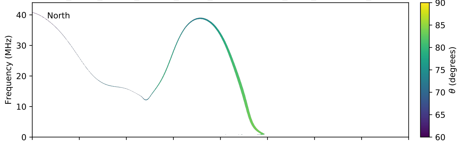
expres_earth_jupiter_europa_jrm09_lossc-wid1deg_3kev_20040206_v11.cdf
