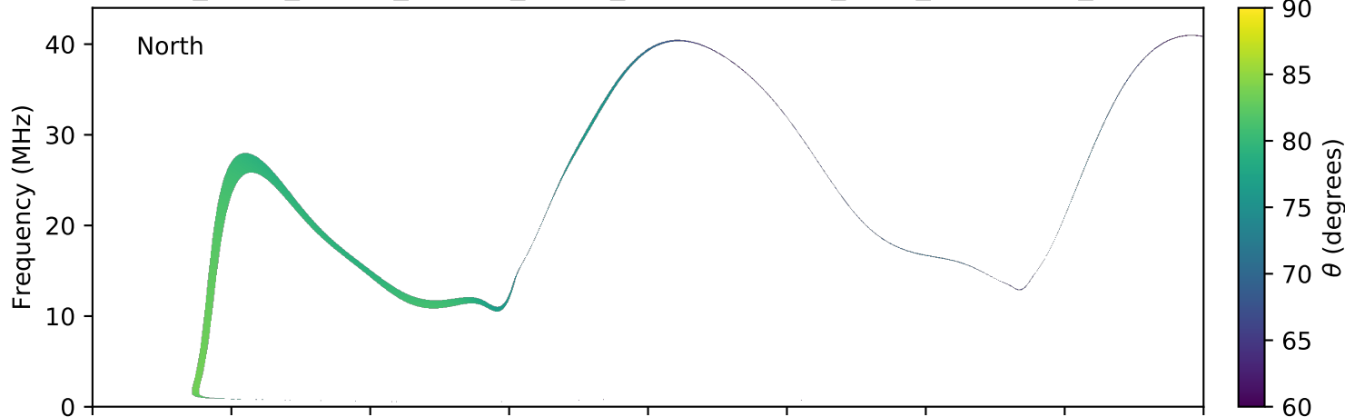
expres_earth_jupiter_europa_jrm09_lossc-wid1deg_3kev_20040205_v11.cdf
