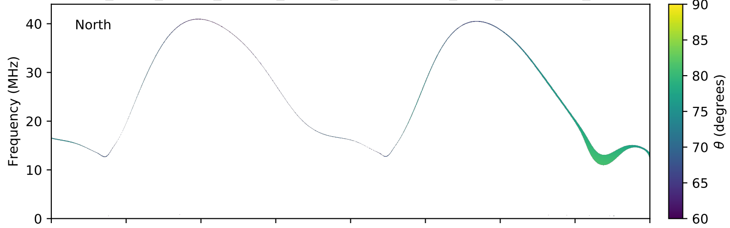
expres_earth_jupiter_europa_jrm09_lossc-wid1deg_3kev_20040202_v11.cdf
