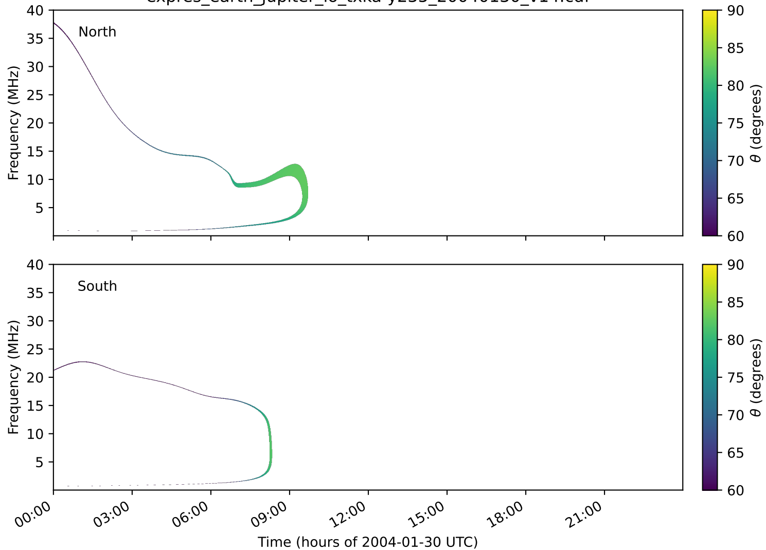
expres_earth_jupiter_io_txka-y235_20040130_v14.cdf
