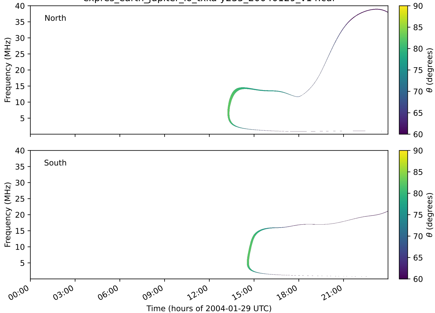
expres_earth_jupiter_io_txka-y235_20040129_v14.cdf
