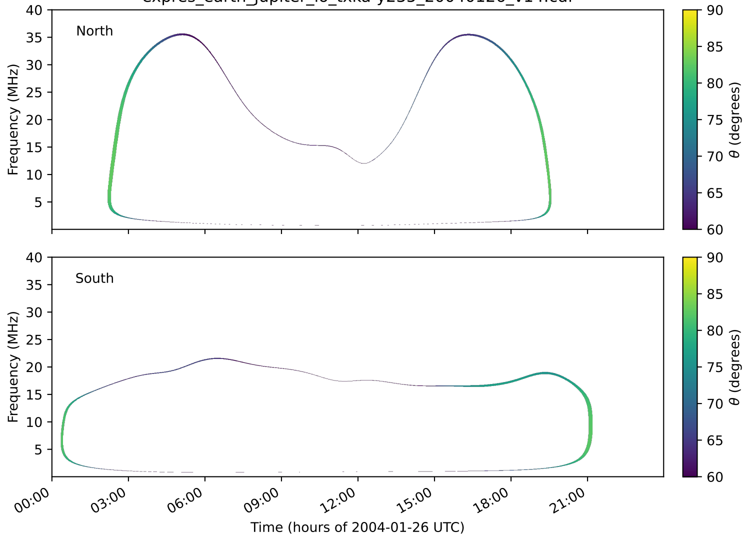
expres_earth_jupiter_io_txka-y235_20040126_v14.cdf
