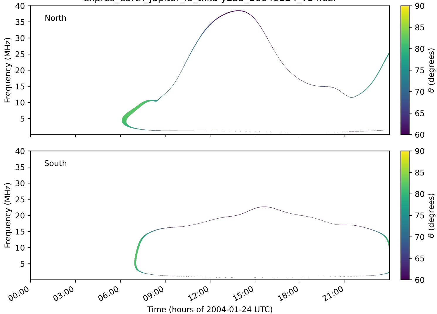
expres_earth_jupiter_io_txka-y235_20040124_v14.cdf
