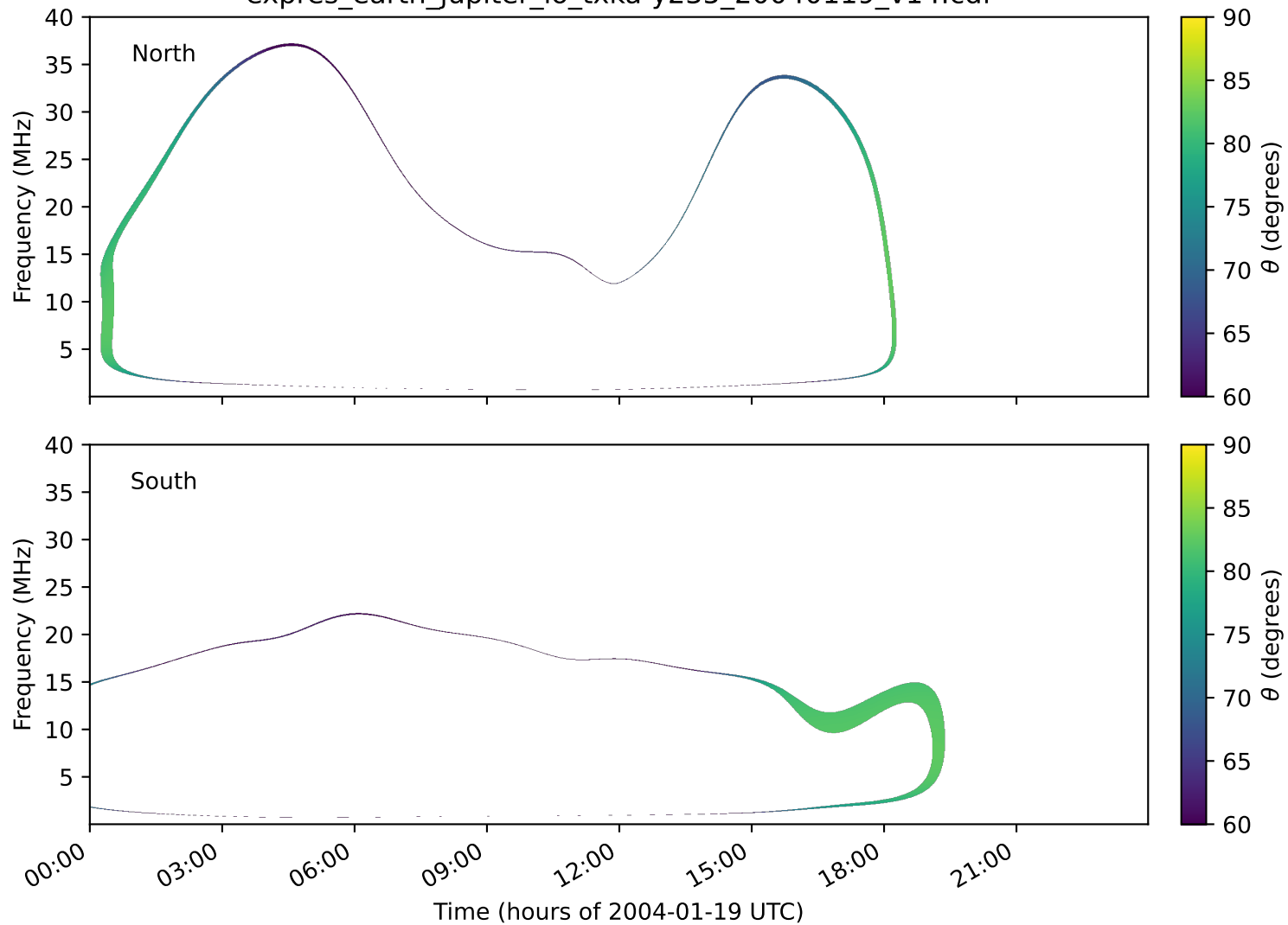
expres_earth_jupiter_io_txka-y235_20040119_v14.cdf
