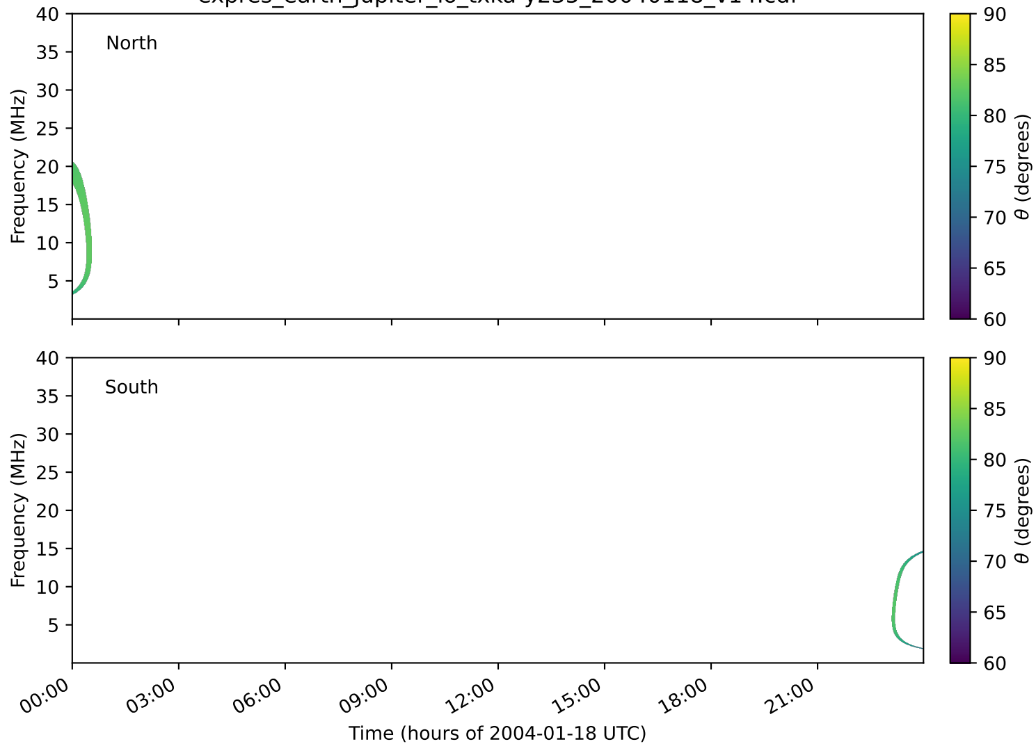
expres_earth_jupiter_io_txka-y235_20040118_v14.cdf
