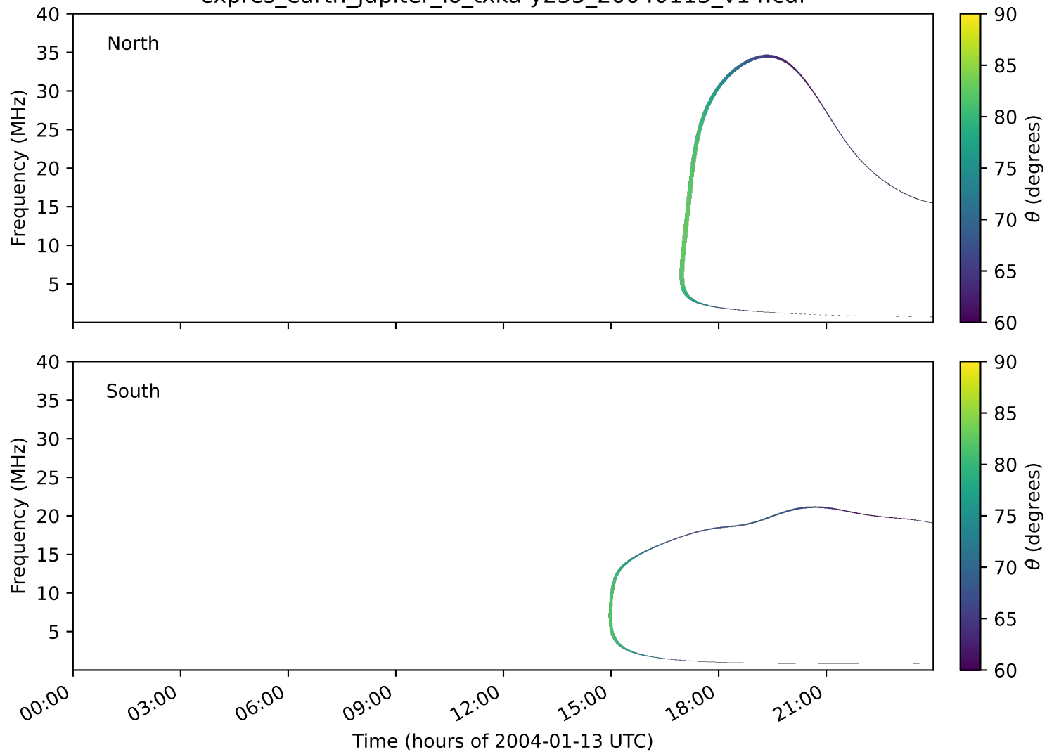
expres_earth_jupiter_io_txka-y235_20040113_v14.cdf
