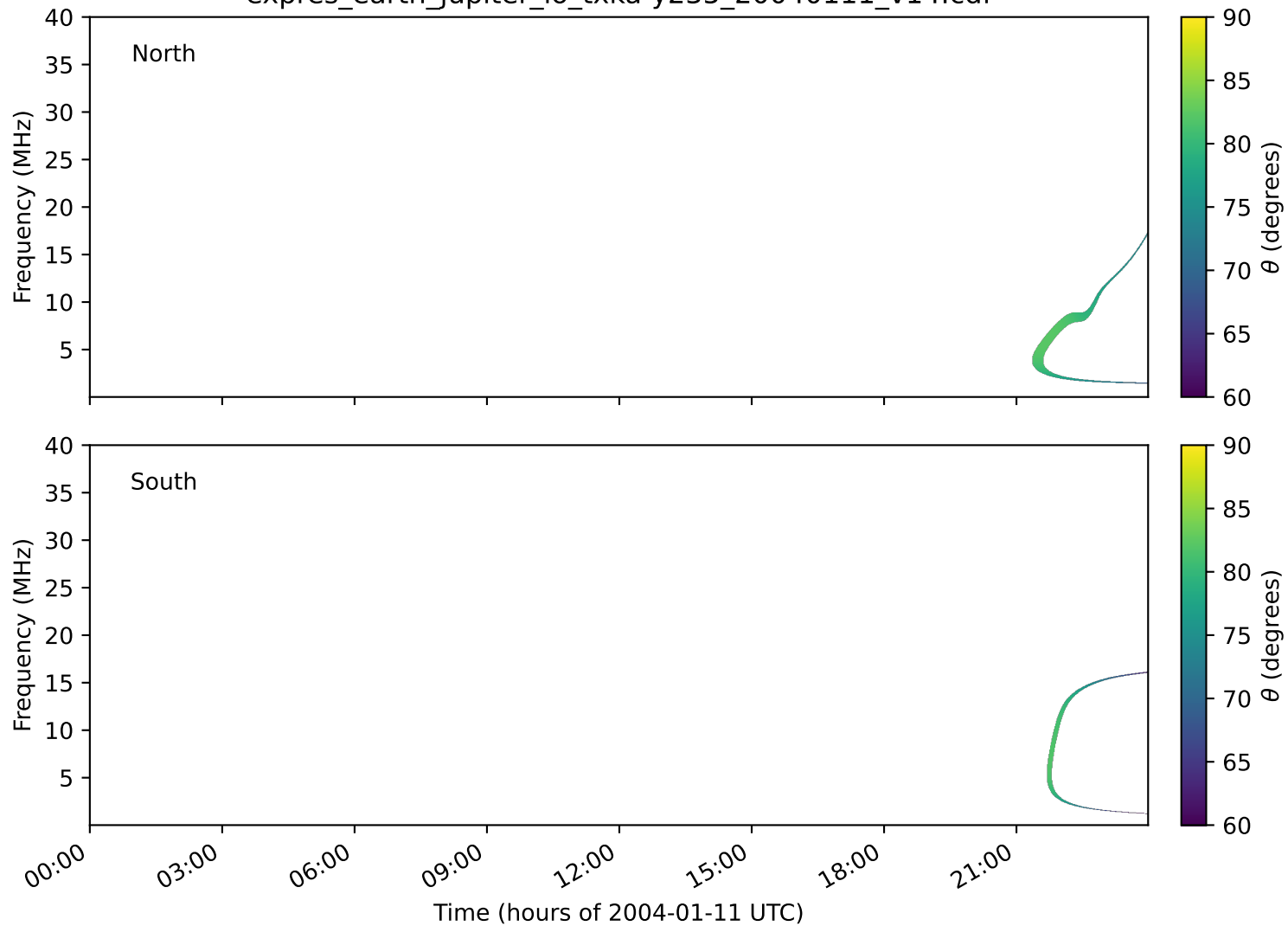
expres_earth_jupiter_io_txka-y235_20040111_v14.cdf
