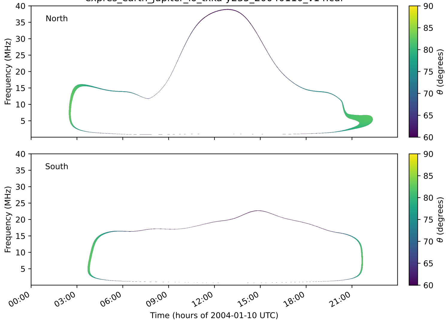
expres_earth_jupiter_io_txka-y235_20040110_v14.cdf
