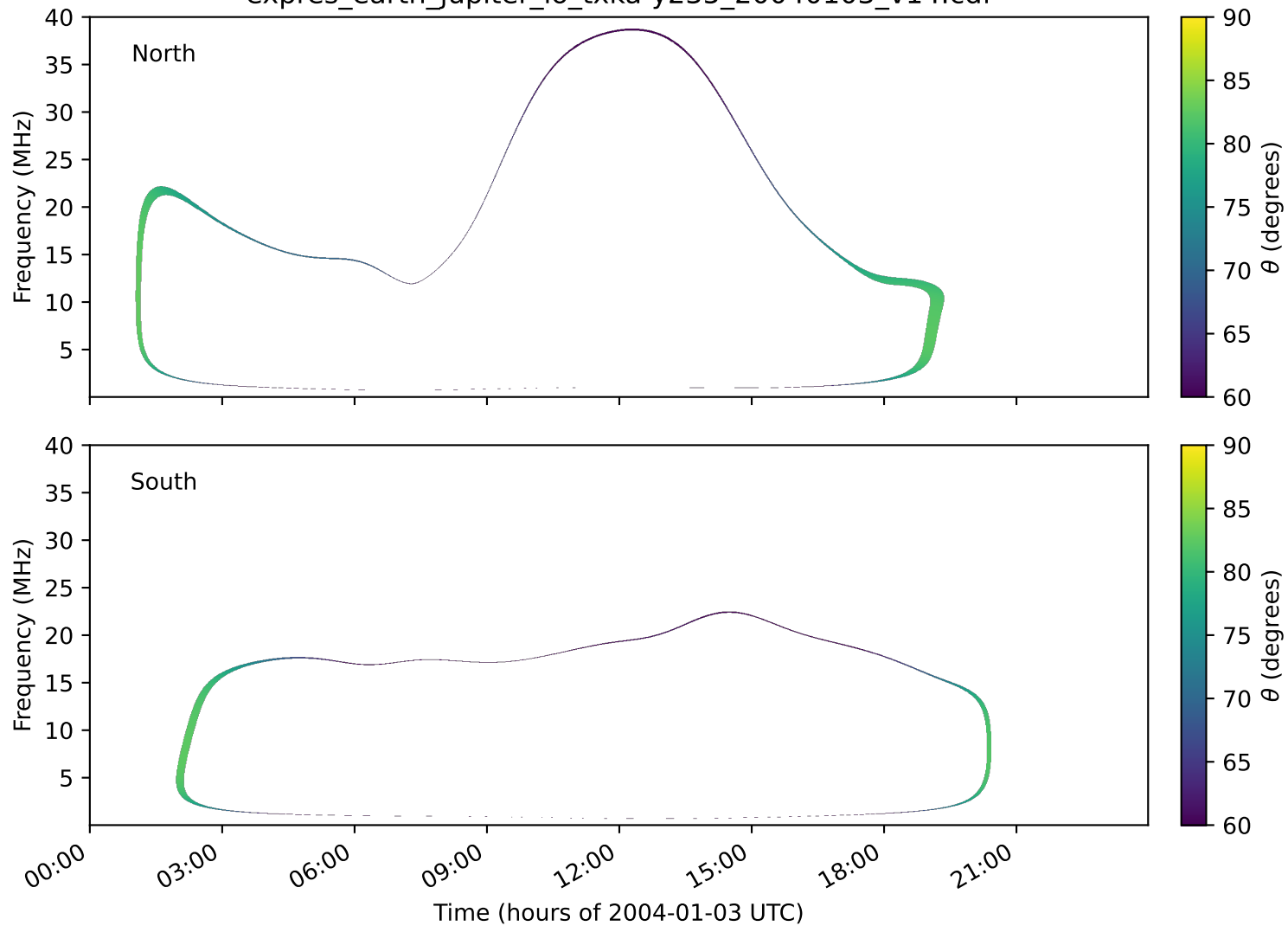
expres_earth_jupiter_io_txka-y235_20040103_v14.cdf
