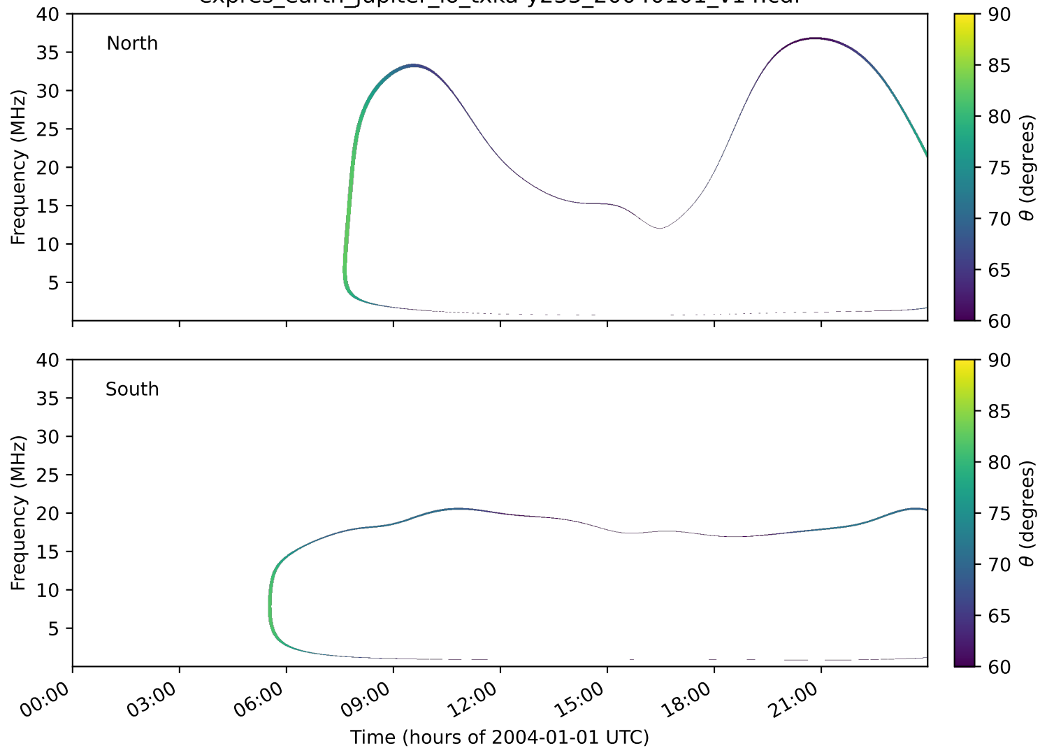
expres_earth_jupiter_io_txka-y235_20040101_v14.cdf
