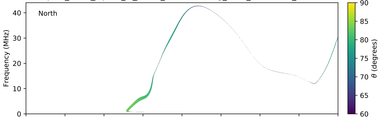
expres_earth_jupiter_io_jrm09_lossc-wid1deg_3kev_20040131_v11.cdf
