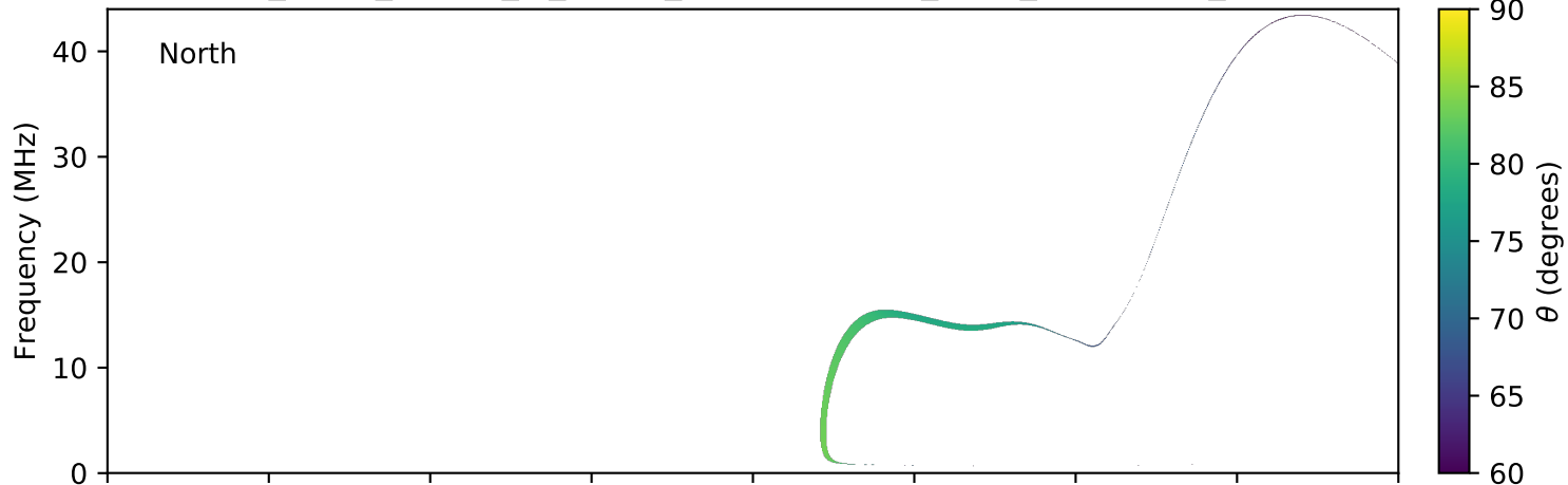
expres_earth_jupiter_io_jrm09_lossc-wid1deg_3kev_20040129_v11.cdf
