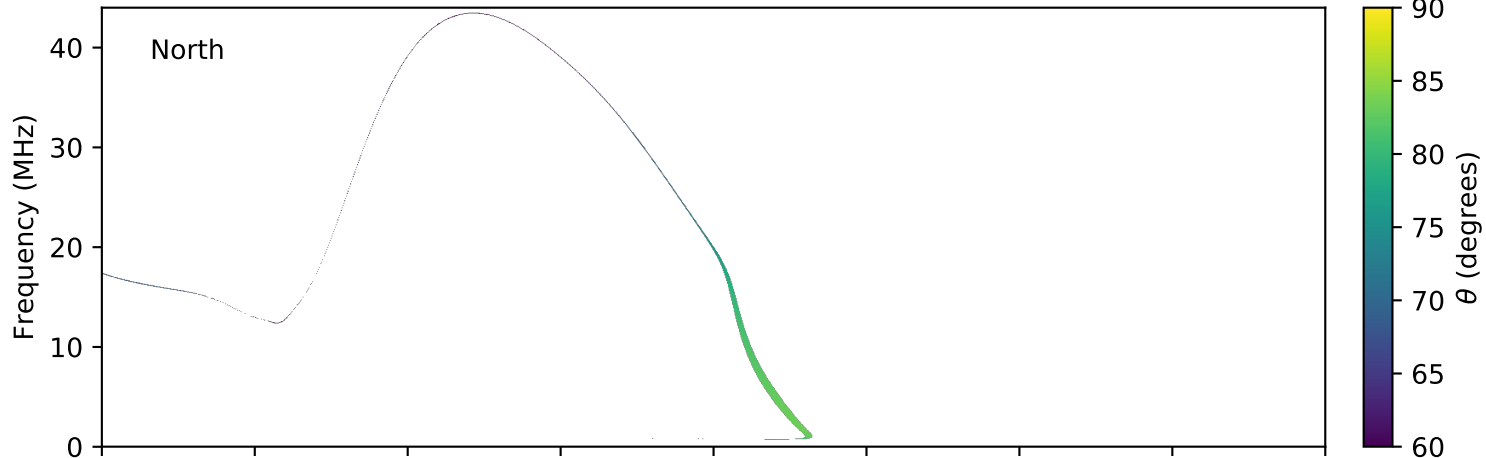
expres_earth_jupiter_io_jrm09_lossc-wid1deg_3kev_20040128_v11.cdf
