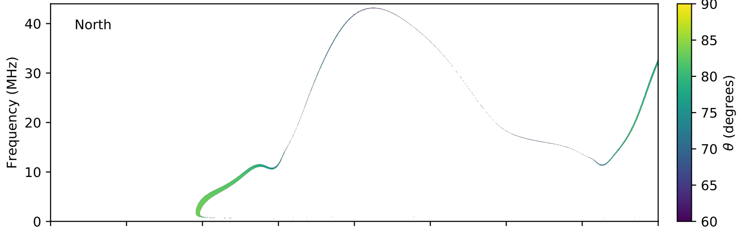
expres_earth_jupiter_io_jrm09_lossc-wid1deg_3kev_20040124_v11.cdf
