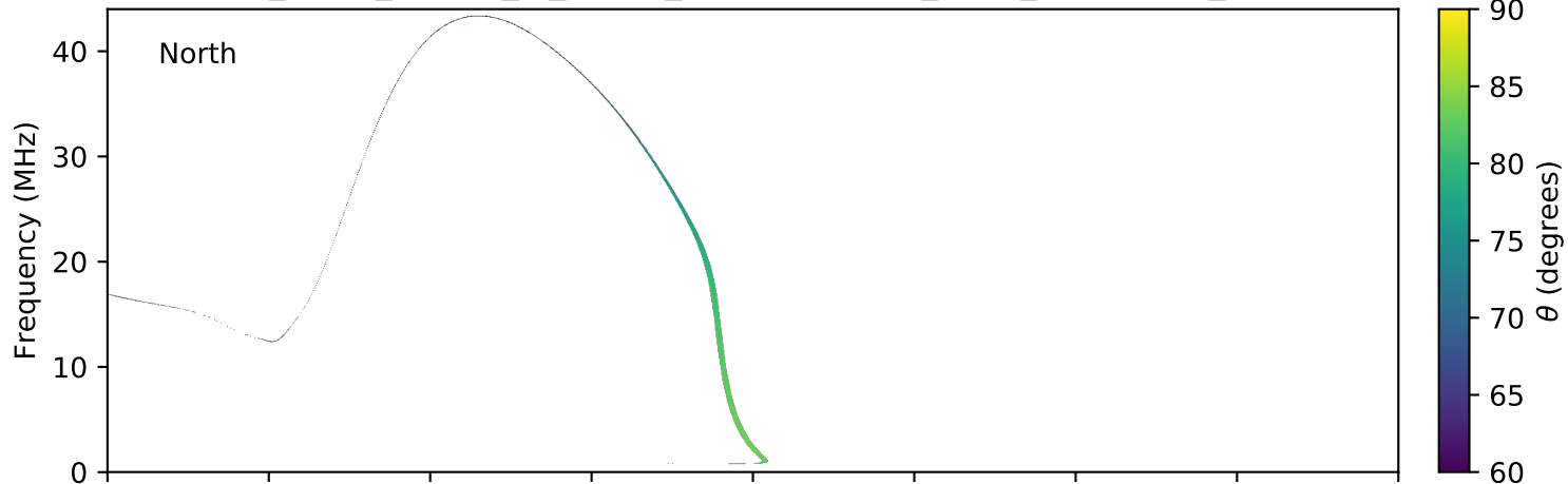
expres_earth_jupiter_io_jrm09_lossc-wid1deg_3kev_20040121_v11.cdf
