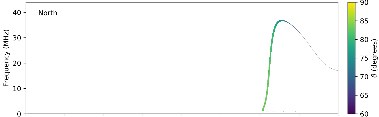
expres_earth_jupiter_io_jrm09_lossc-wid1deg_3kev_20040120_v11.cdf
