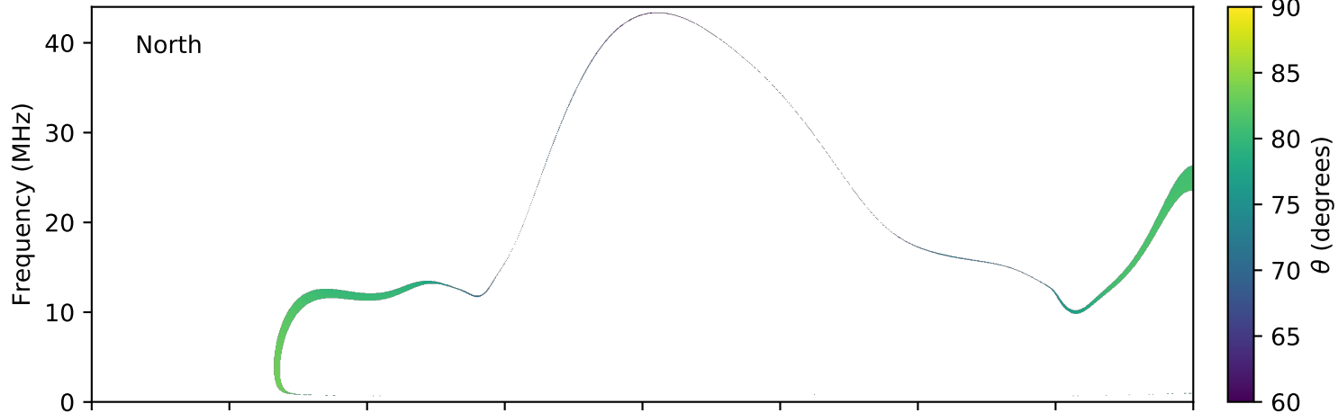
expres_earth_jupiter_io_jrm09_lossc-wid1deg_3kev_20040117_v11.cdf
