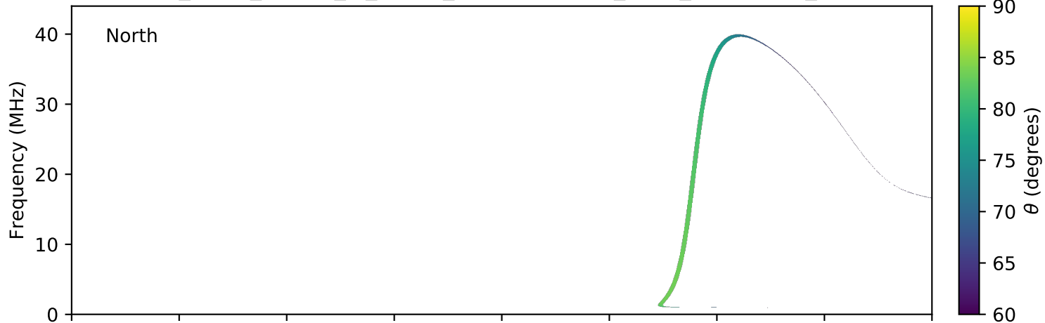
expres_earth_jupiter_io_jrm09_lossc-wid1deg_3kev_20040113_v11.cdf
