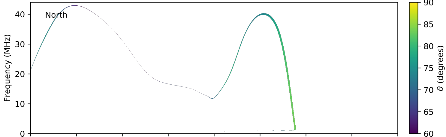
expres_earth_jupiter_io_jrm09_lossc-wid1deg_3kev_20040112_v11.cdf
