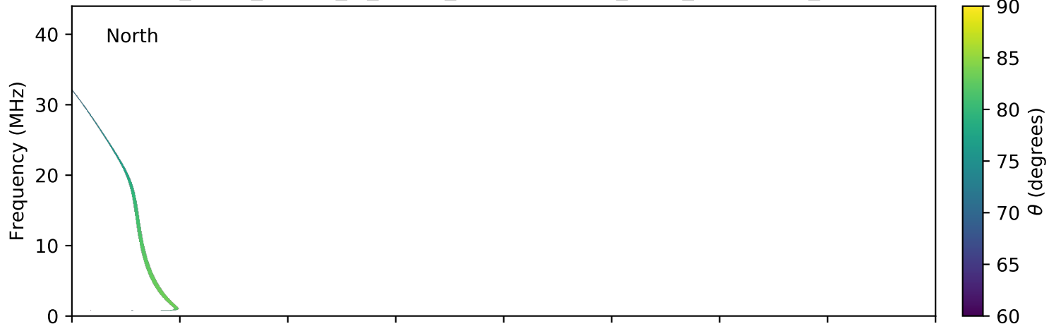
expres_earth_jupiter_io_jrm09_lossc-wid1deg_3kev_20040109_v11.cdf
