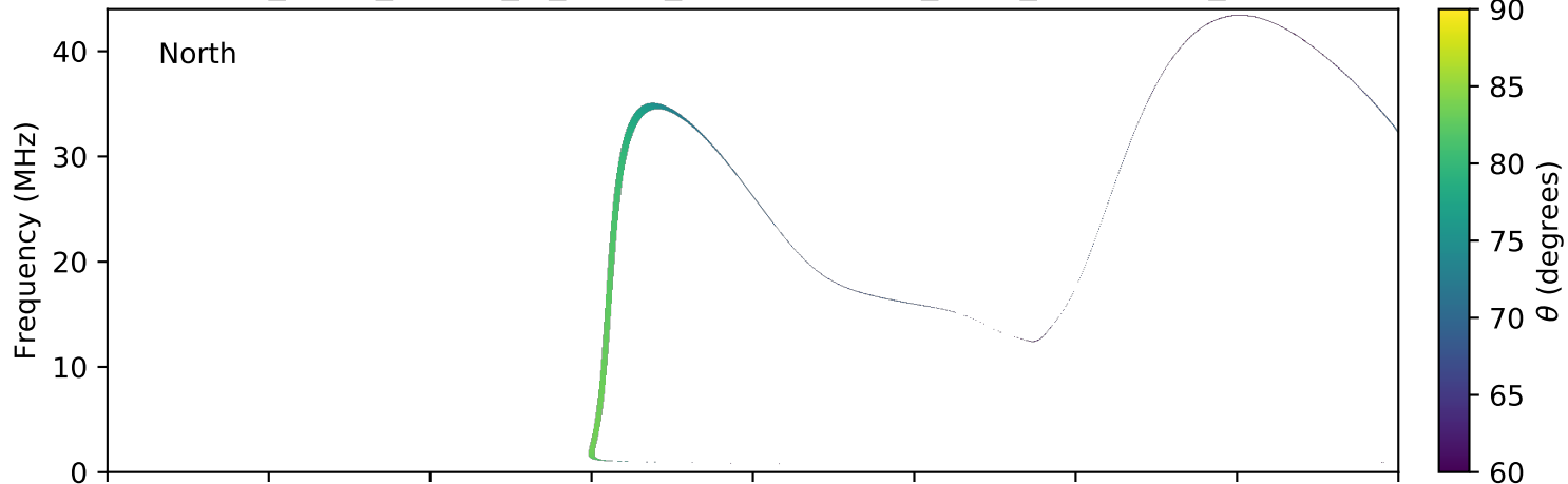
expres_earth_jupiter_io_jrm09_lossc-wid1deg_3kev_20040108_v11.cdf
