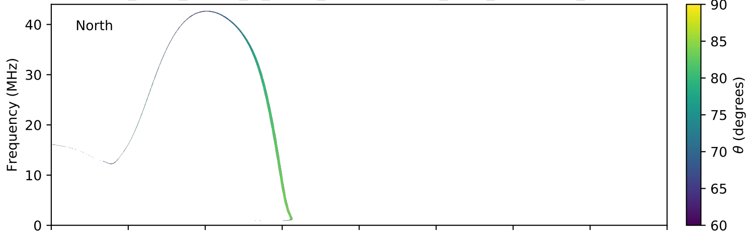
expres_earth_jupiter_io_jrm09_lossc-wid1deg_3kev_20040107_v11.cdf
