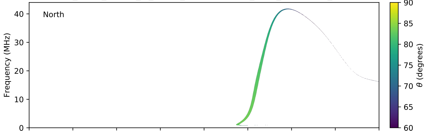
expres_earth_jupiter_io_jrm09_lossc-wid1deg_3kev_20040106_v11.cdf
