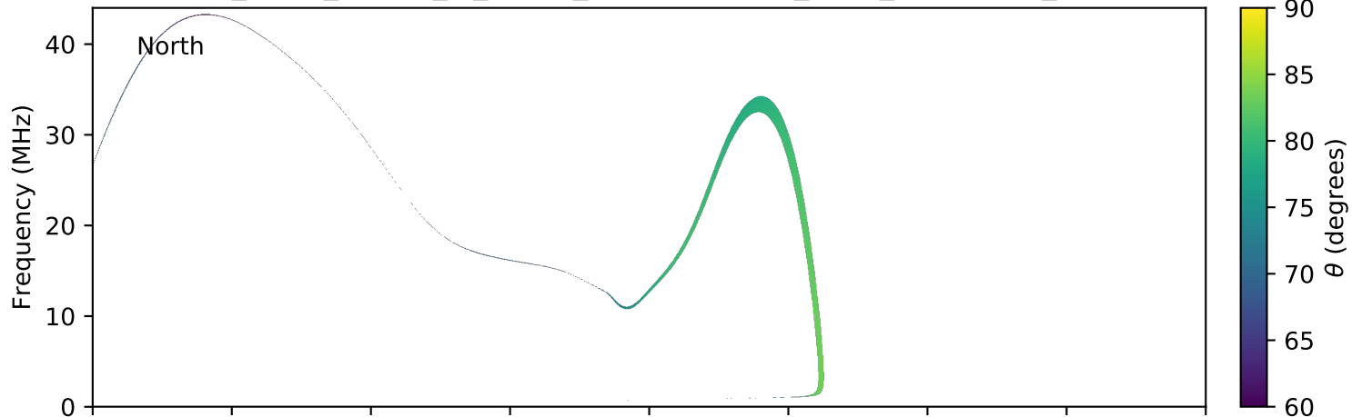
expres_earth_jupiter_io_jrm09_lossc-wid1deg_3kev_20040105_v11.cdf
