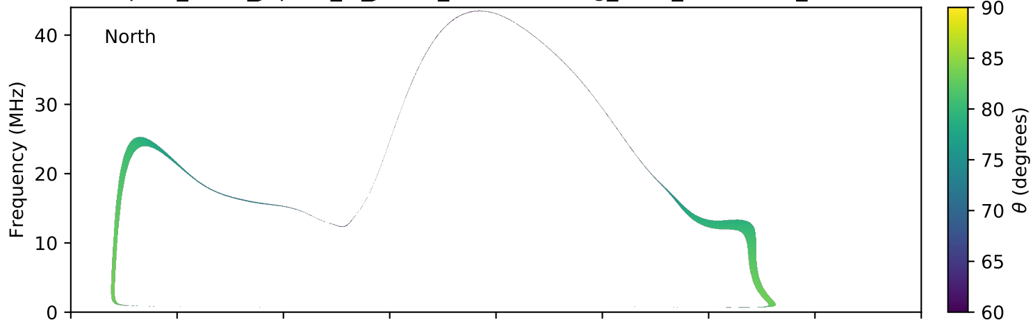
expres_earth_jupiter_io_jrm09_lossc-wid1deg_3kev_20040103_v11.cdf
