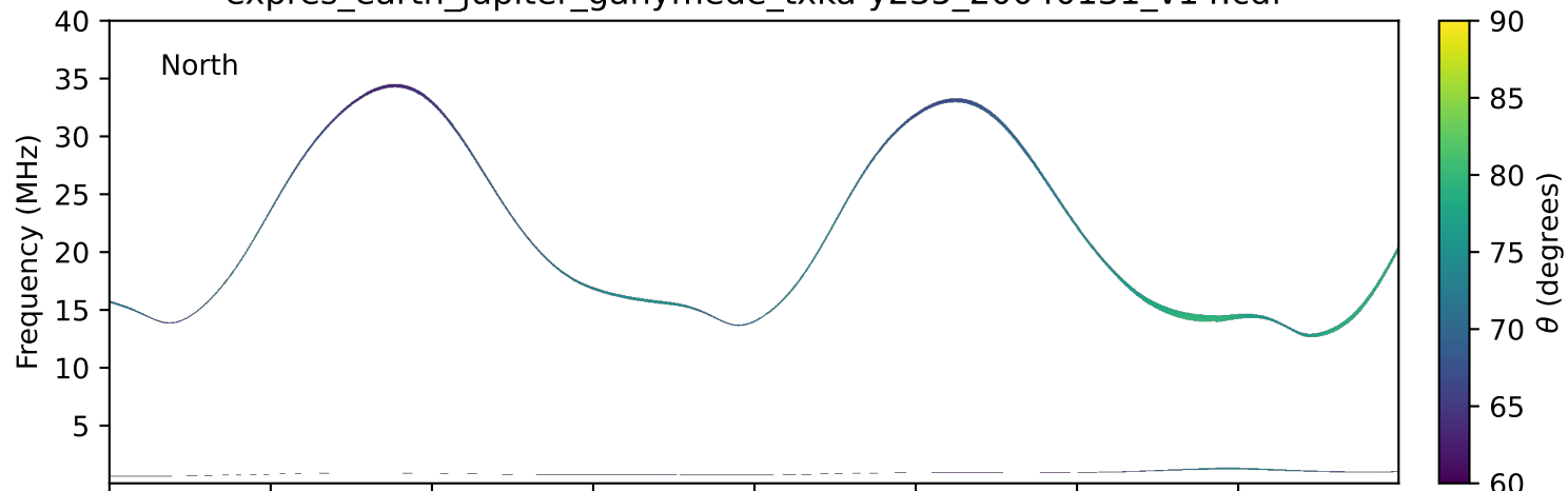
expres_earth_jupiter_ganymede_txka-y235_20040131_v14.cdf
