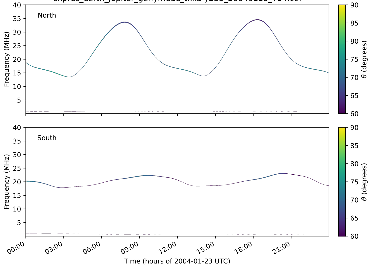
expres_earth_jupiter_ganymede_txka-y235_20040123_v14.cdf
