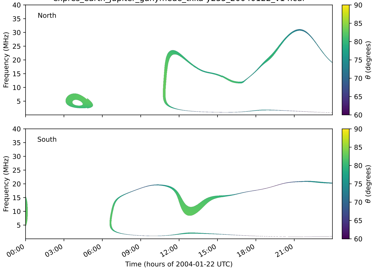
expres_earth_jupiter_ganymede_txka-y235_20040122_v14.cdf
