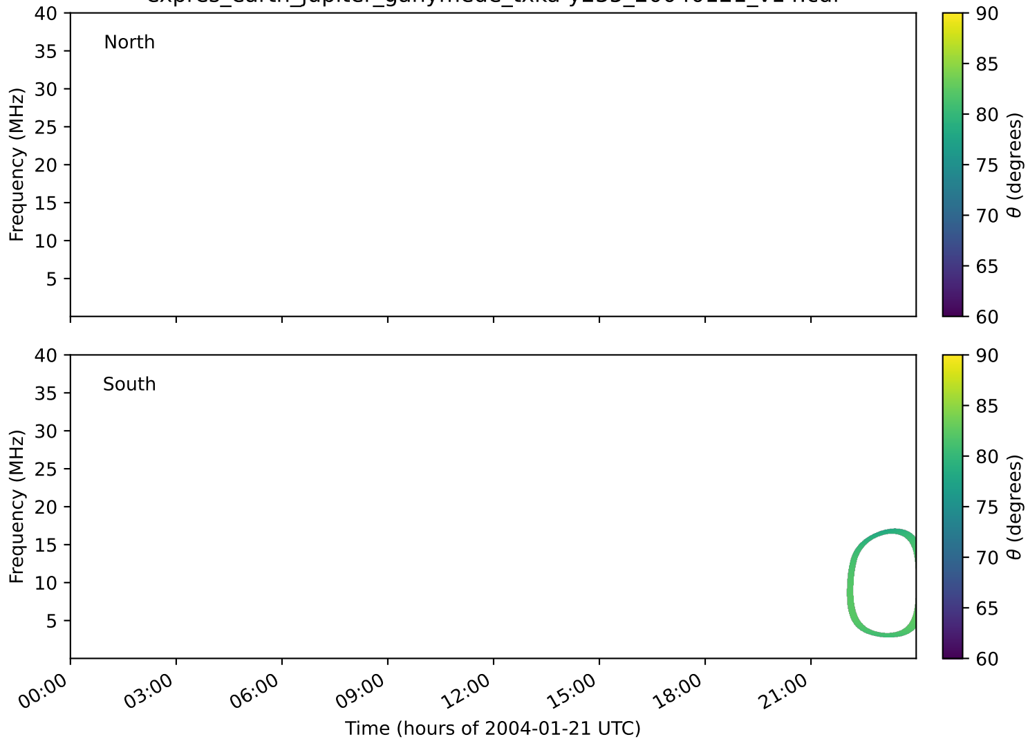
expres_earth_jupiter_ganymede_txka-y235_20040121_v14.cdf
