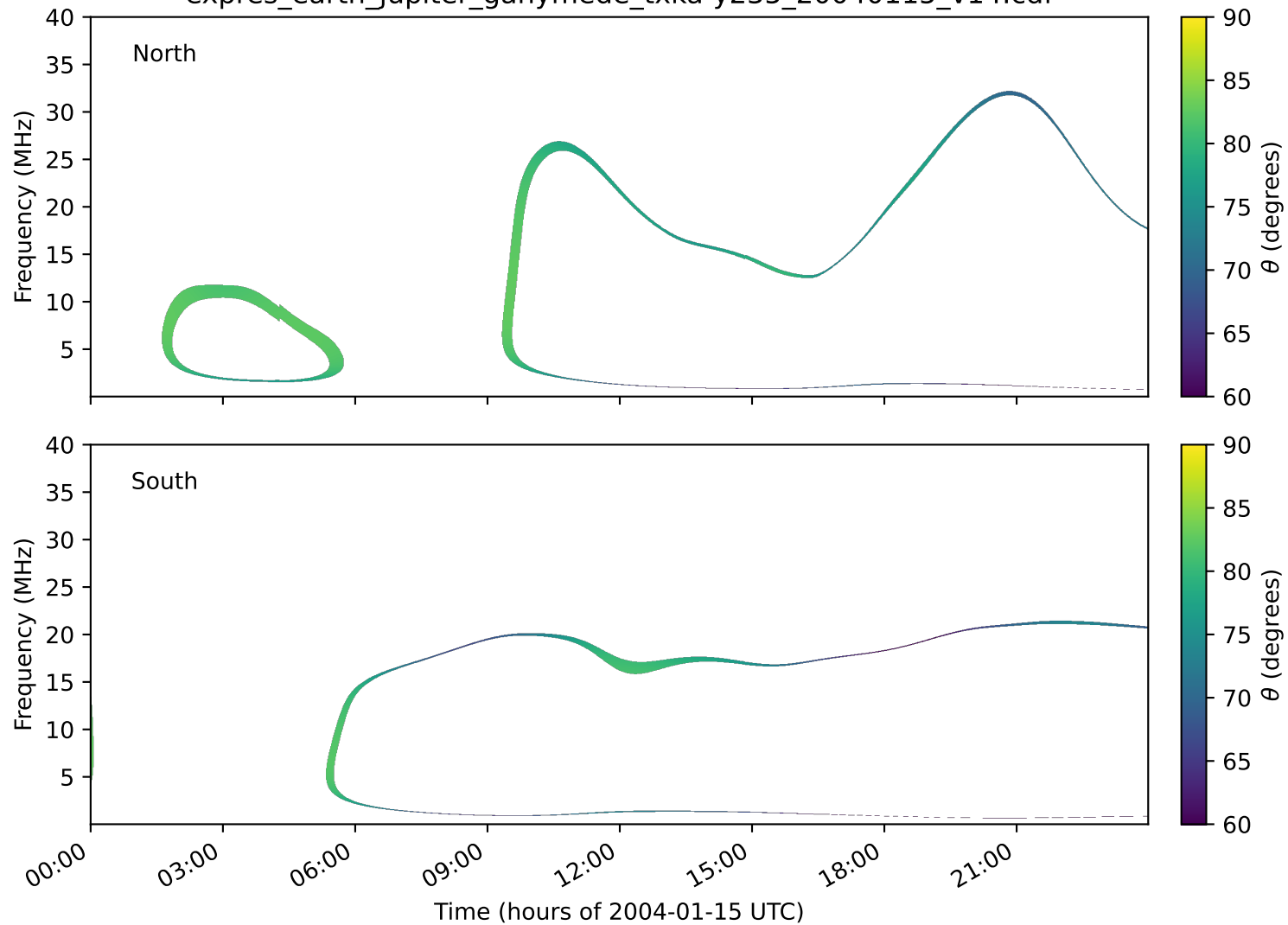
expres_earth_jupiter_ganymede_txka-y235_20040115_v14.cdf
