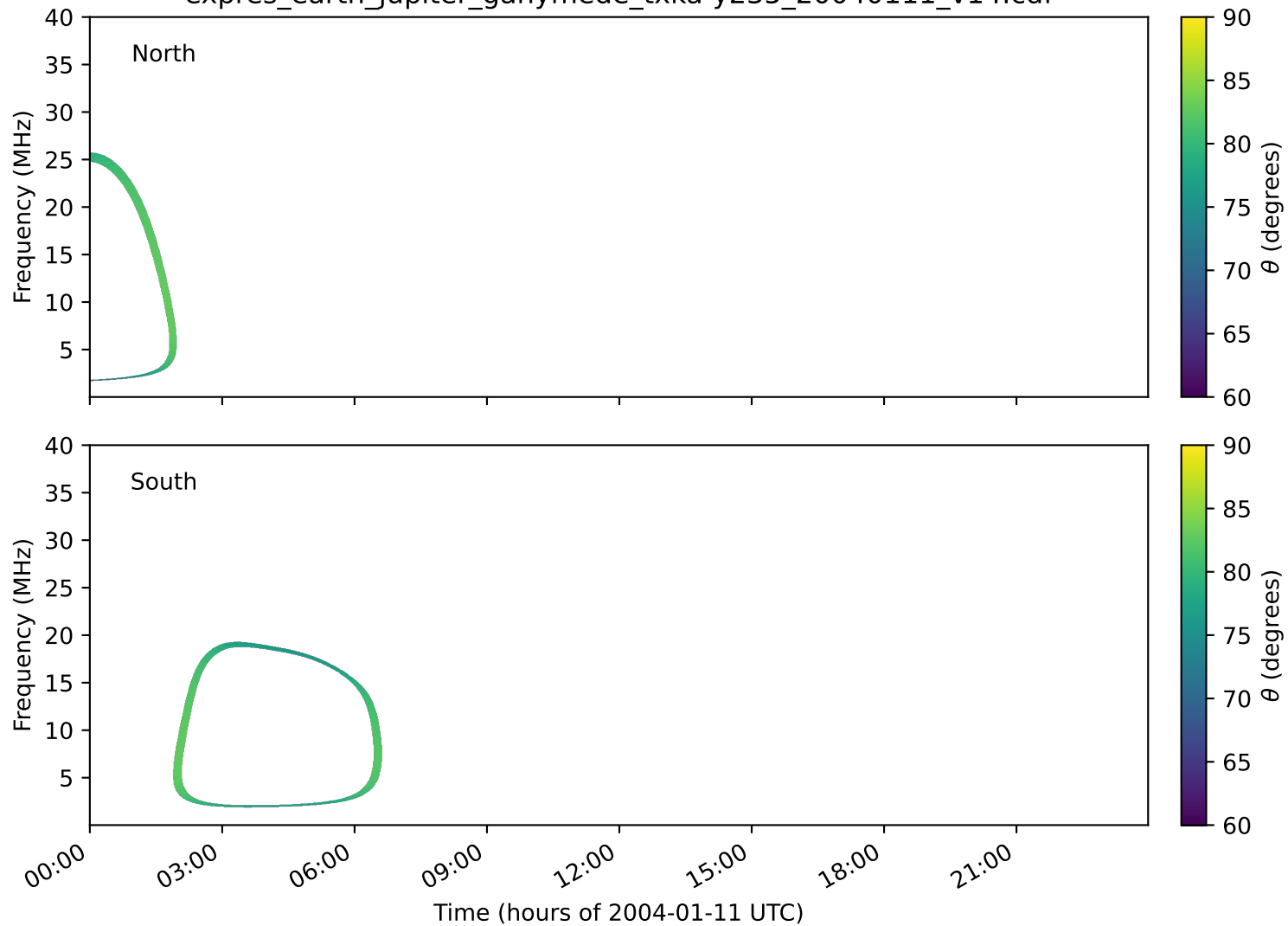
expres_earth_jupiter_ganymede_txka-y235_20040111_v14.cdf
