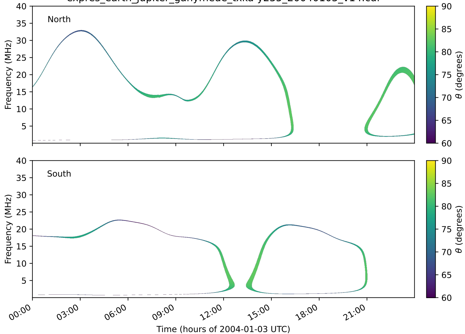
expres_earth_jupiter_ganymede_txka-y235_20040103_v14.cdf
