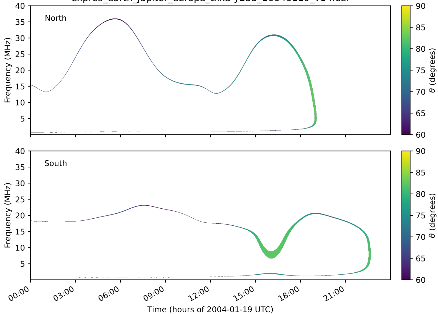
expres_earth_jupiter_europa_txka-y235_20040119_v14.cdf
