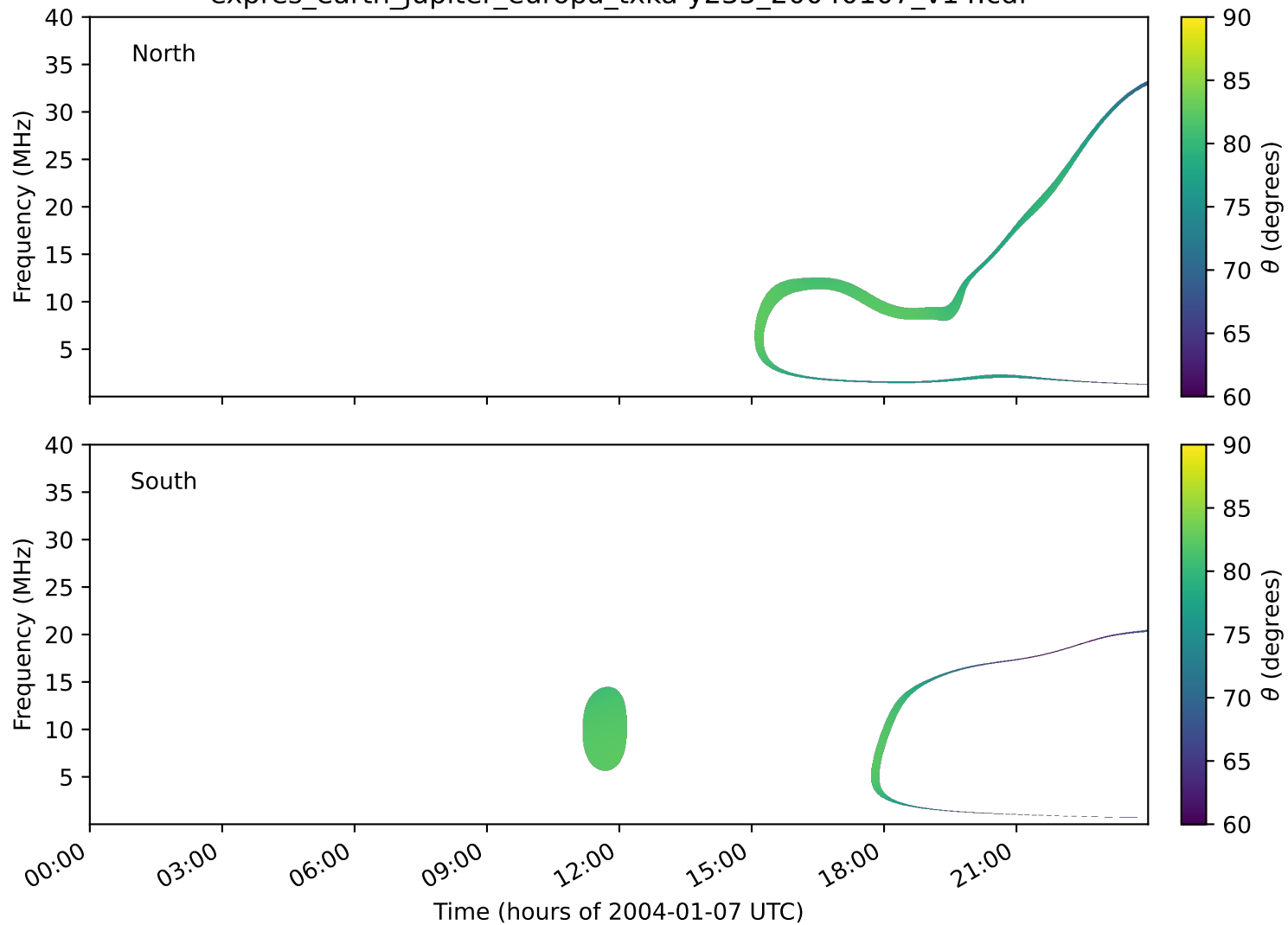
expres_earth_jupiter_europa_txka-y235_20040107_v14.cdf
