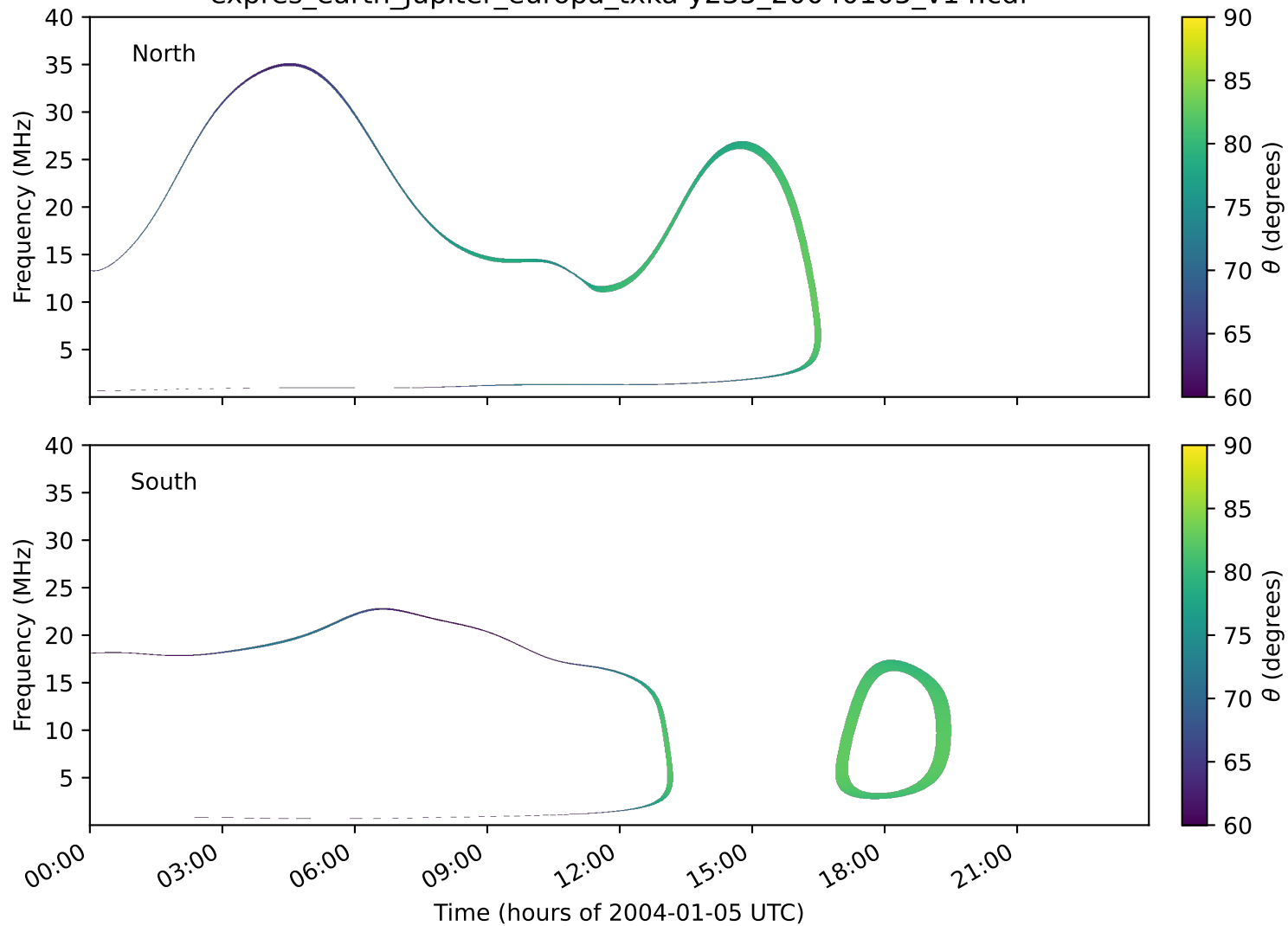
expres_earth_jupiter_europa_txka-y235_20040105_v14.cdf
