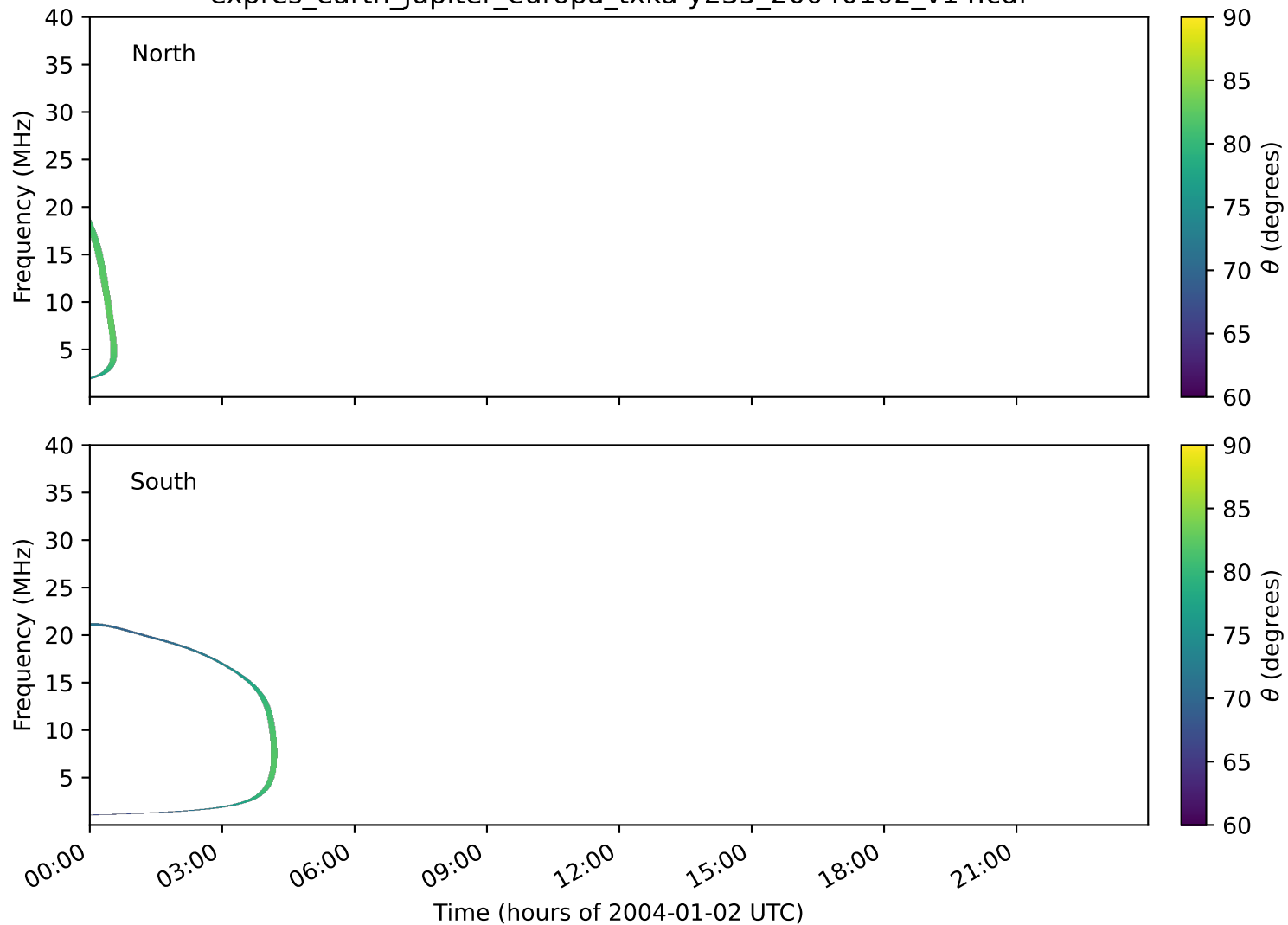
expres_earth_jupiter_europa_txka-y235_20040102_v14.cdf
