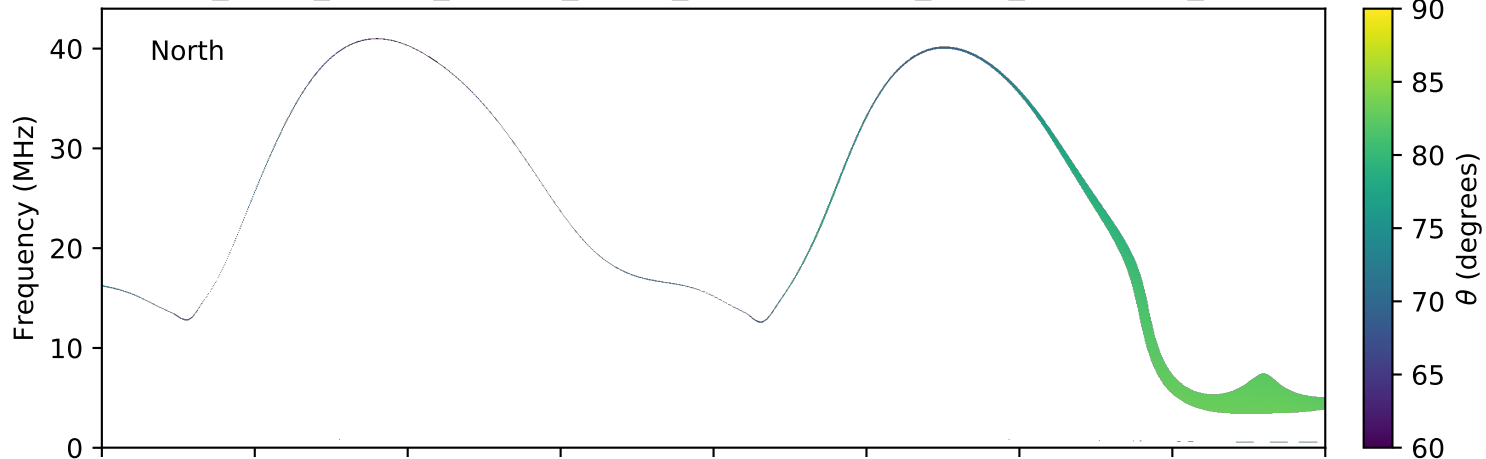
expres_earth_jupiter_europa_jrm09_lossc-wid1deg_3kev_20040126_v11.cdf
