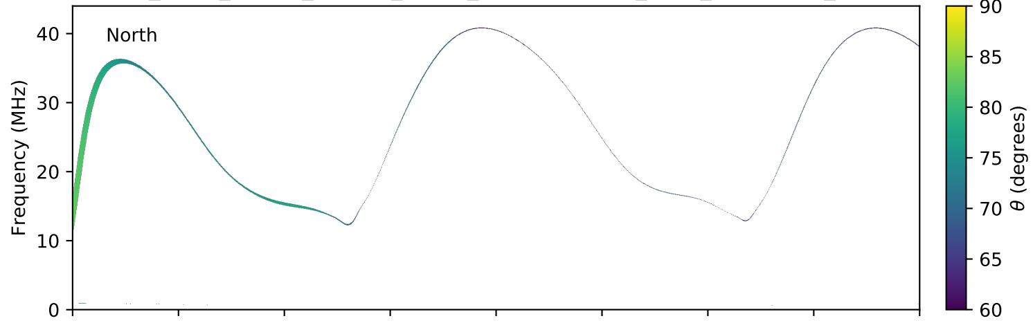
expres_earth_jupiter_europa_jrm09_lossc-wid1deg_3kev_20040122_v11.cdf
