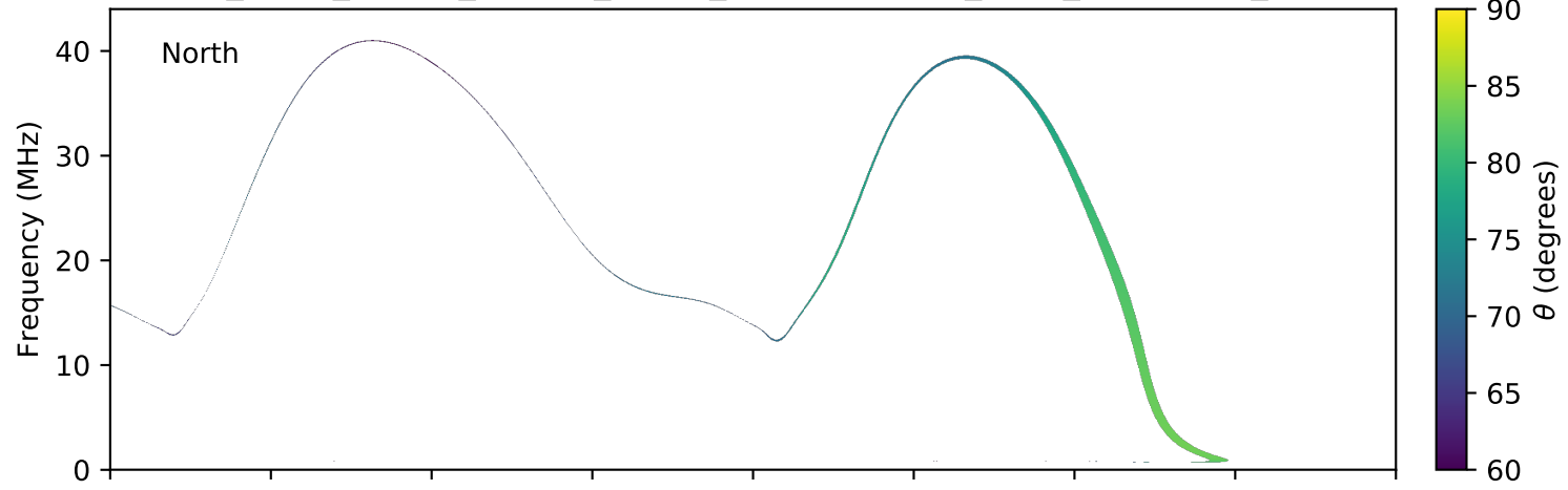
expres_earth_jupiter_europa_jrm09_lossc-wid1deg_3kev_20040119_v11.cdf
