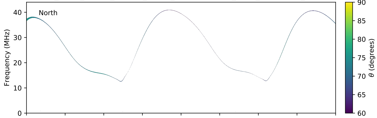
expres_earth_jupiter_europa_jrm09_lossc-wid1deg_3kev_20040115_v11.cdf
