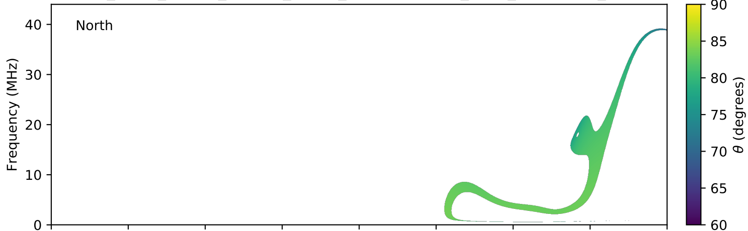
expres_earth_jupiter_europa_jrm09_lossc-wid1deg_3kev_20040107_v11.cdf
