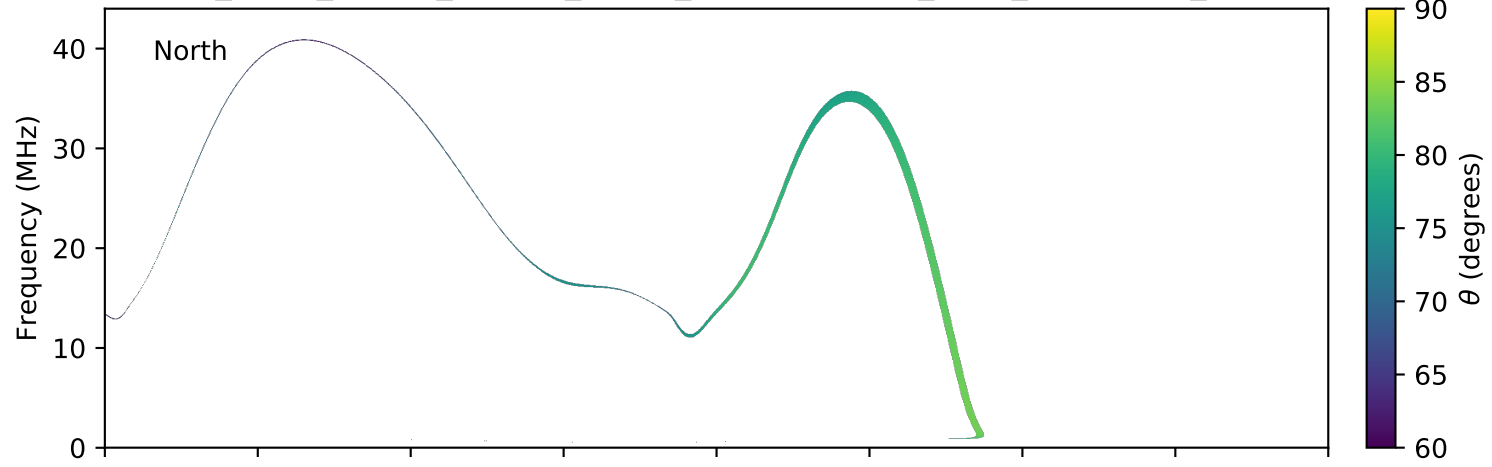
expres_earth_jupiter_europa_jrm09_lossc-wid1deg_3kev_20040105_v11.cdf
