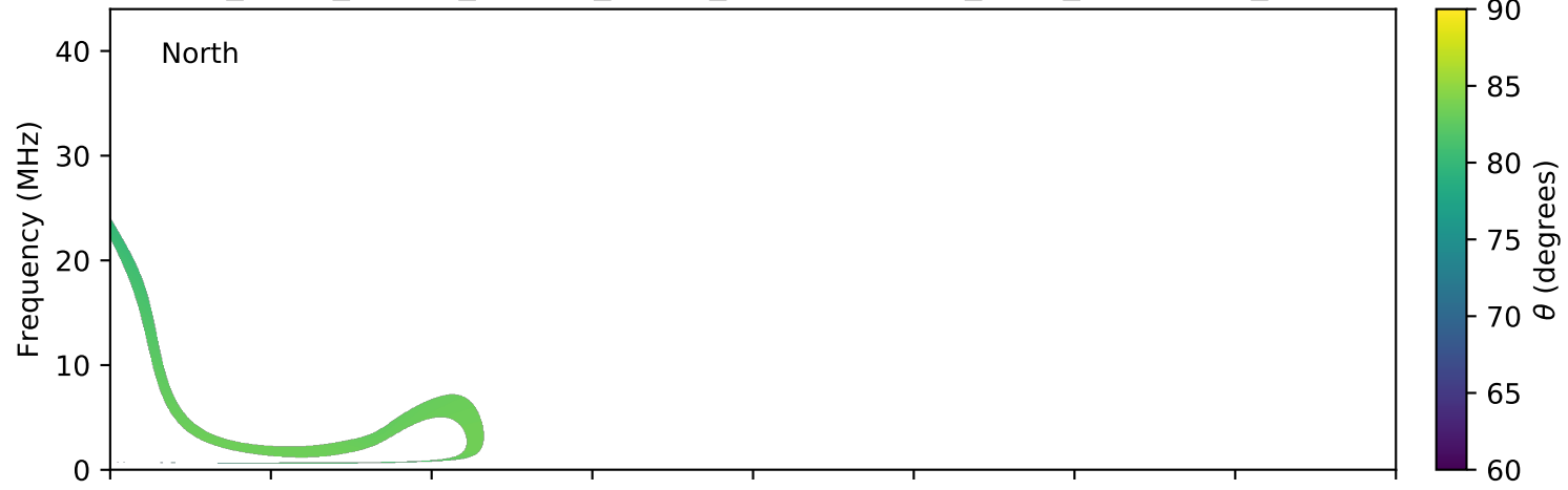
expres_earth_jupiter_europa_jrm09_lossc-wid1deg_3kev_20040102_v11.cdf
