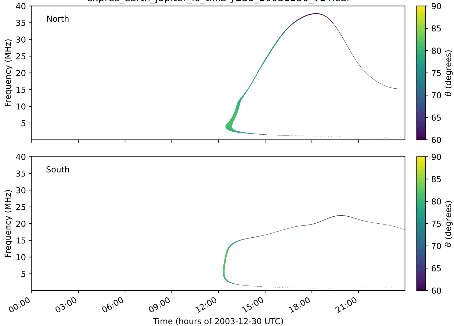
expres_earth_jupiter_io_txka-y235_20031230_v14.cdf
